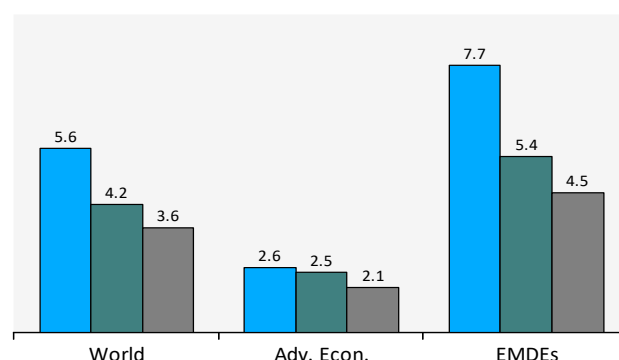
Figure 2: Global Inflation
