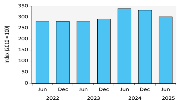
Figure 8: Manufacturing Index
