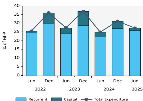
Figure 14: Government Expenditure
