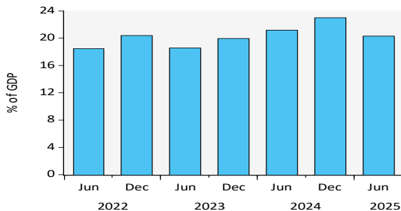
Figure 6: Liquidity
